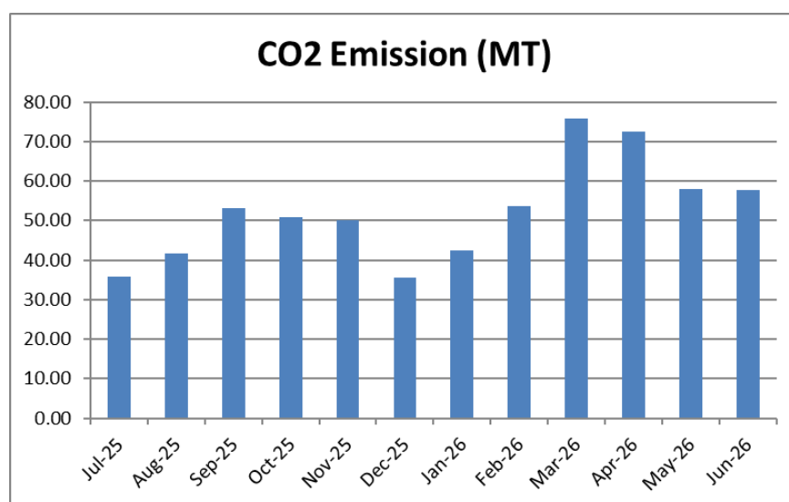
Figure 4.1: Month wise CO2 Emission
